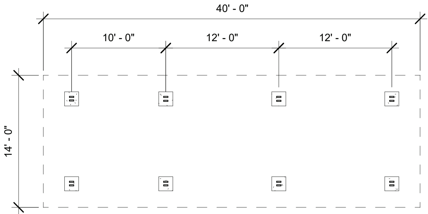
floor plan
