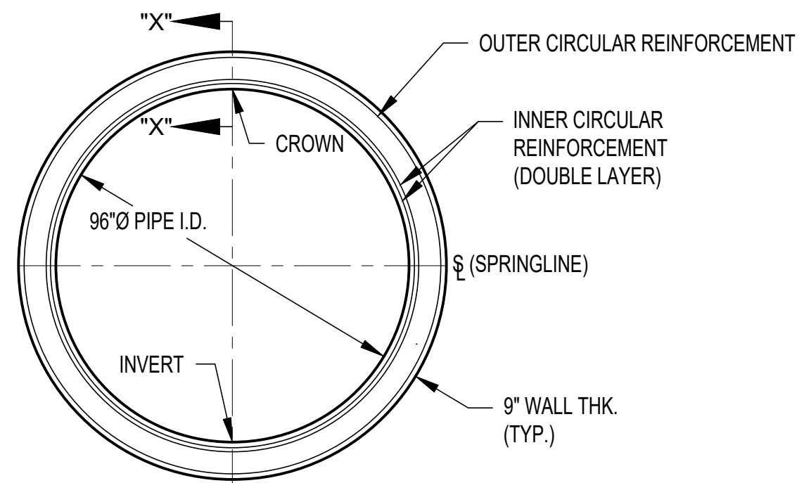
SECTION "Y"-"Y": THRU BARREL
